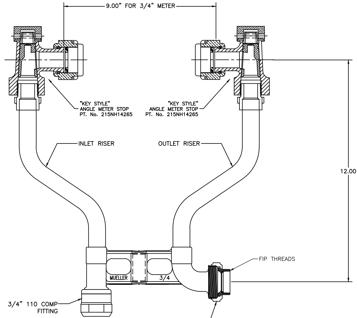
MULTI-PURPOSE CONNECTION WITH H14222N INSTALLED
