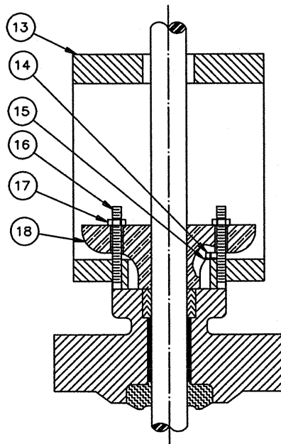
REPLACEABLE PACKING AND BONNET ASSEMBLY (WHEN REQ'D)
