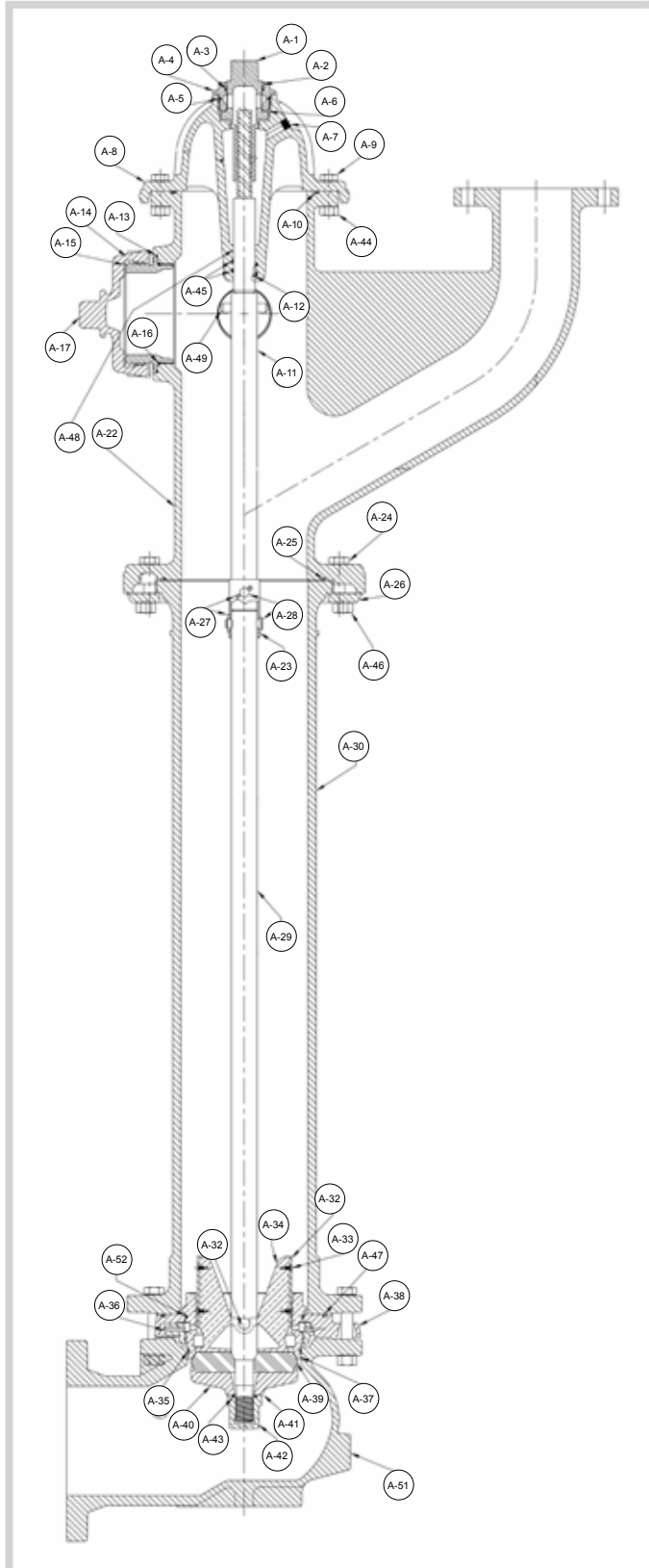
5 1/4" UL/FM Mueller Super Centurion Monitor Fire Hydrant replacement parts
