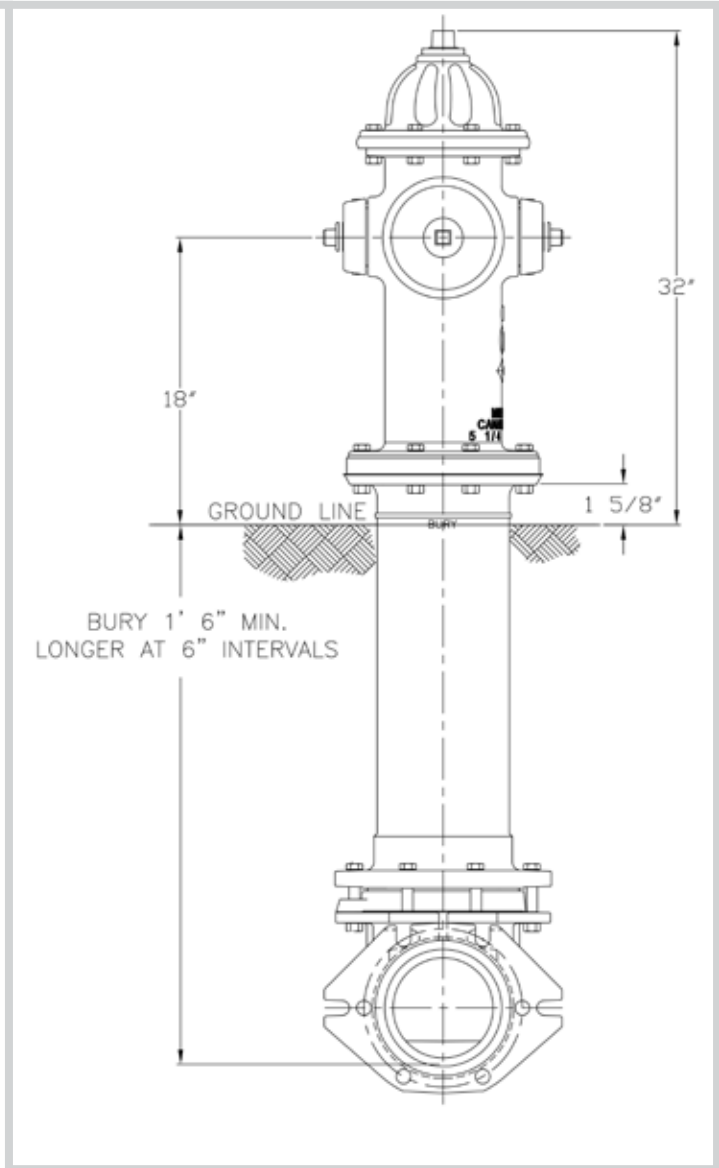
5 1/4" UL/FM Mueller Super Centurion Monitor Fire Hydrant replacement parts
