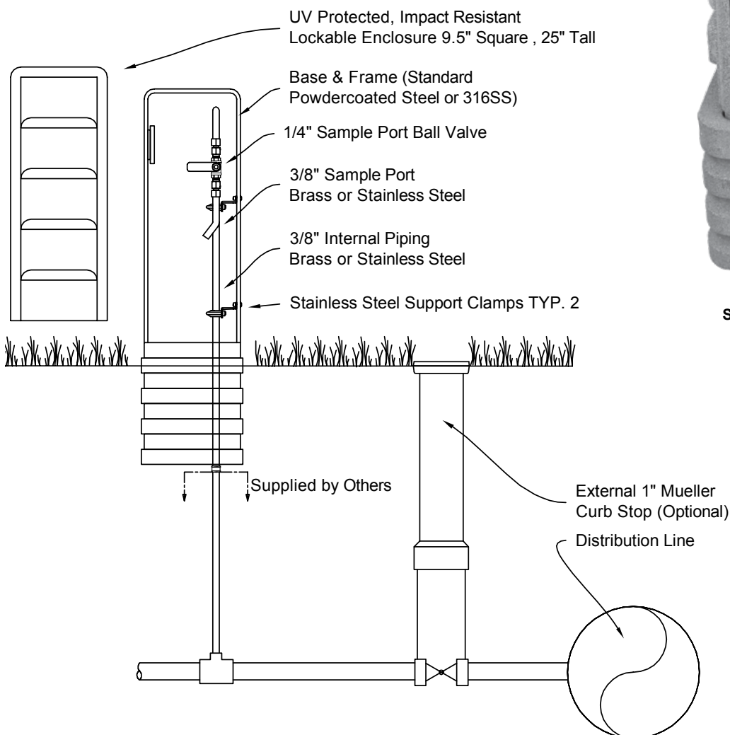
BSS05-CHA-00-SP Cold Climate Sample Station Installation (typ)
