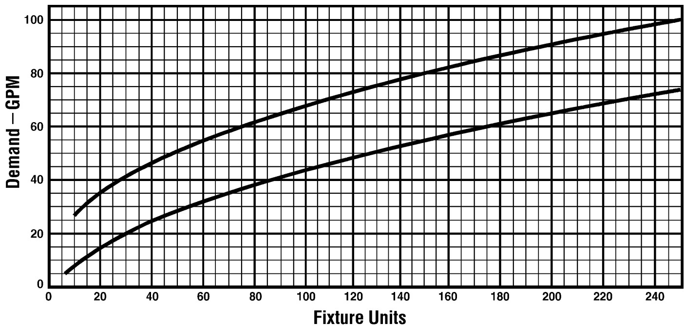
Figure 8 - Chart of demand weights in fixture units
