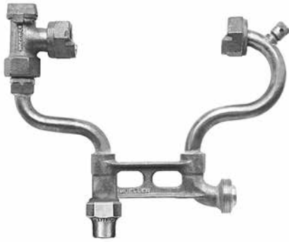
Integral copper flare vertical inlet and horizontal outlet with multi-purpose connection (H-1483N shown)
