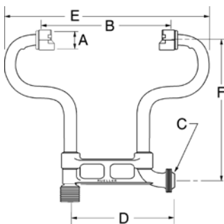
M-98™ ASSE approved top entry vertical check valve
