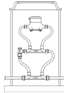
Typical installation of a relocater type horizontal inlet and outlet copper meter yoke
