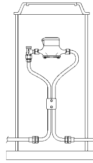
Typical installation of a flexible relocater type copper meter yoke
