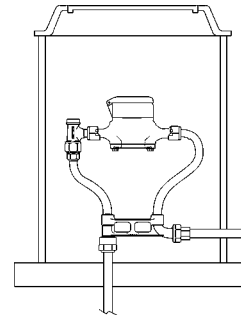
Typical installation of a vertical inlet and horizontal outlet copper meter yoke
