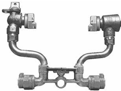
Mueller Pack Joint Connection ends (P-2542-2AN)
