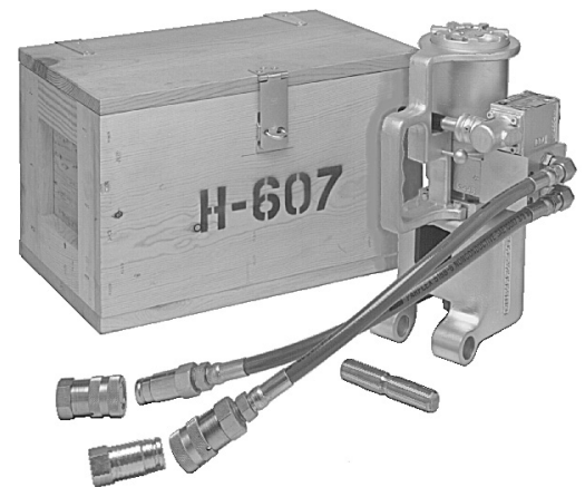
H-607 hydraulic power operator
