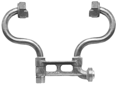
MIP vertical inlet and horizontal outlet with multi-purpose connection (H-1568 shown)
