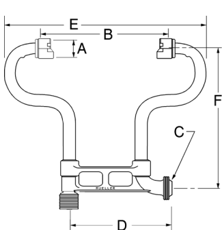
M-98™ ASSE approved top entry vertical check valve
