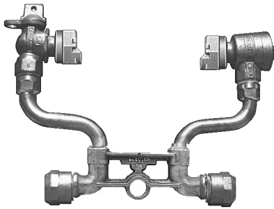
MUELLER 110 ® Conductive Compression ends (B-2470-2A)
