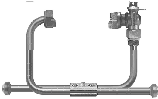
Multi-purpose thread ends (B-2706 shown)
