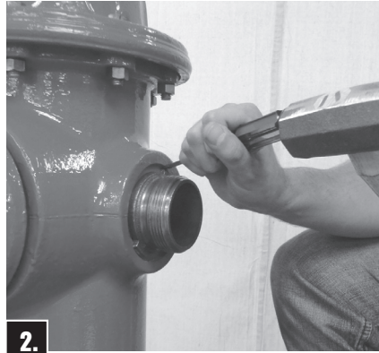
2. Remove stainless steel Nozzle Lock by driving it out with a pointed tool and hammer.
