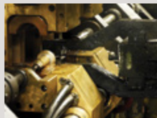
STEM IS ELECTRICALLY HEATED AND THRUST TOGETHER TO CREATE THE THRUST COLLAR
