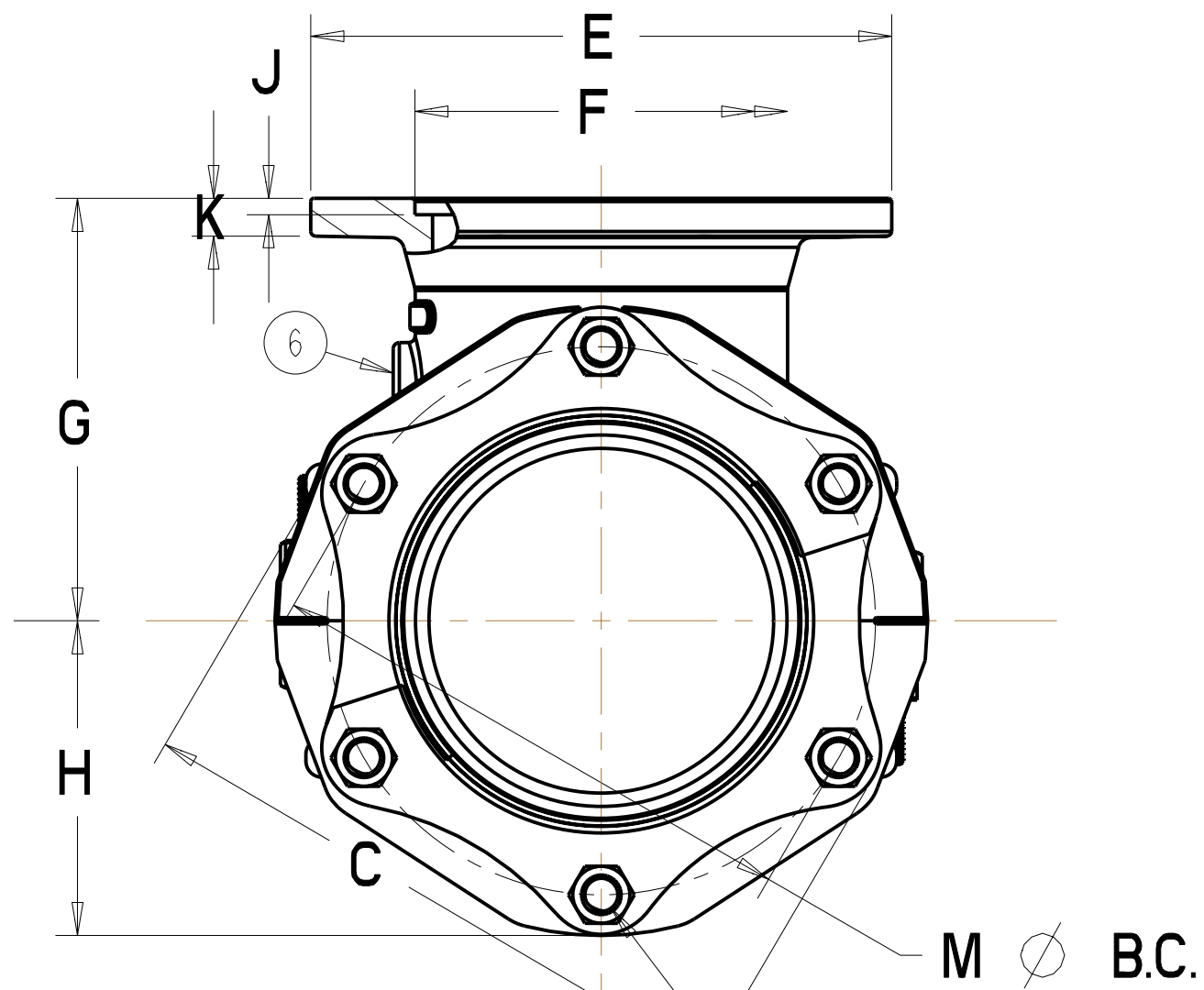
SECTION E-E
