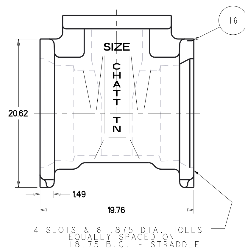
MECHANICAL JOINT ENDS
