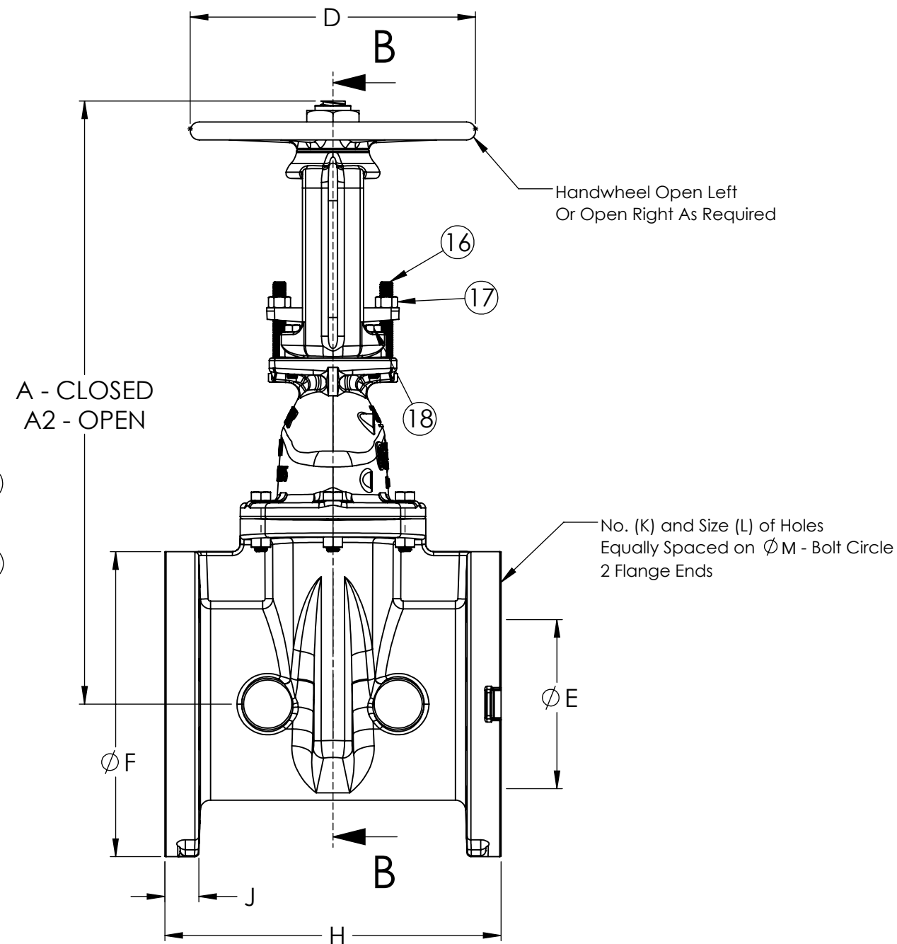
DIMENSIONS FOR RESILIENT WEDGE GATE VALVES - INCHES
