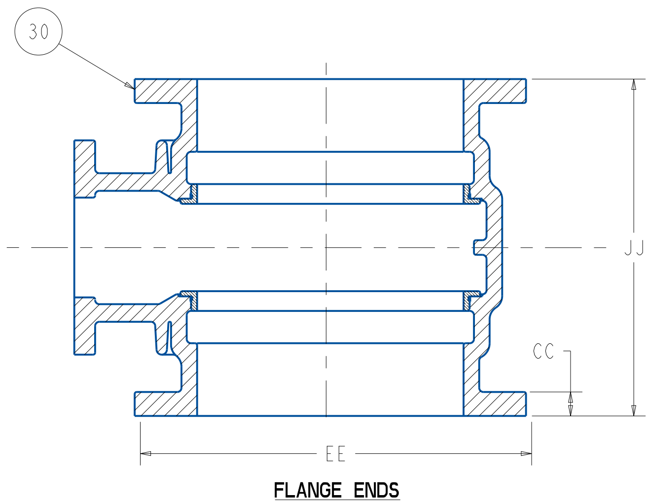
FLANGE ENDS
