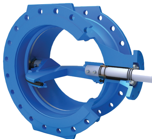
DN100 - DN250 SINGLE SHAFT DESIGN
