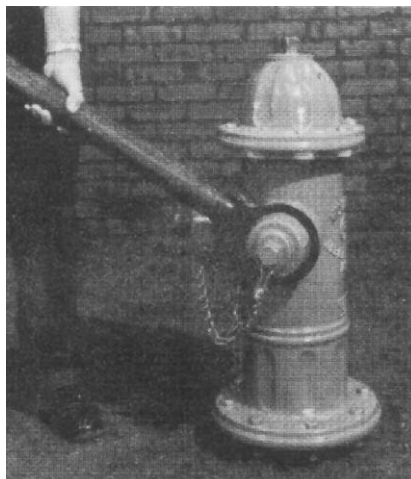
4. Remove Nozzle. The Nozzle Wrench may be struck with a heavy brass hammer or additional leverage may be obtained by placing a length of 2" schedule 40 steel pipe over the handle of the Nozzle Wrench.
