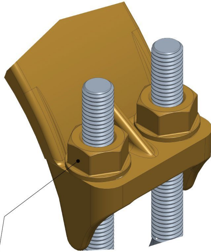
"FN" OPTION FLANGE NUT CAST BRASS ALLOY 83600 / FORGED BRASS ALLOY C69300
