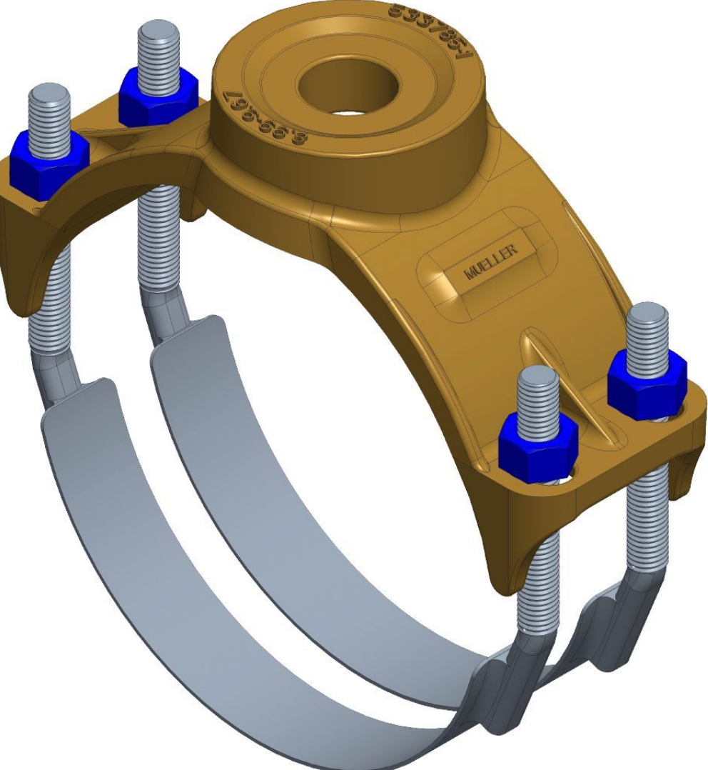
LARGE BOSS SADDLE TAPS 1.25"-2.00"
