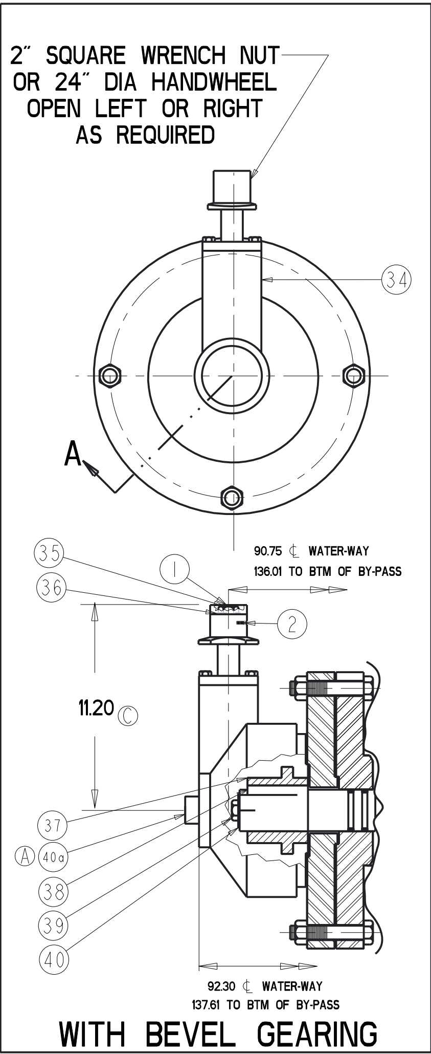
SECTION A SPUR/BEVEL GEARING
